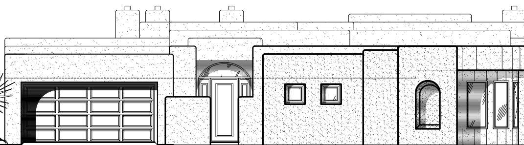
SOUTH ELEVATION SCALE = 1/4" = 1'-0"
