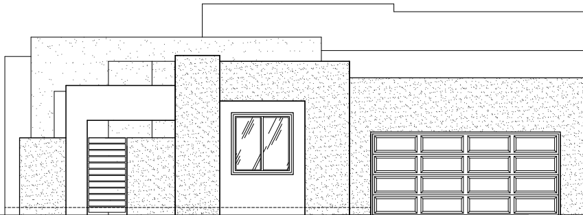
WEST ELEVATION
